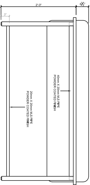
BACK ELEVATION
