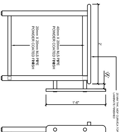
SIDE ELEVATION
